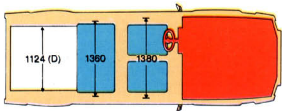
Banquette AR position normale
